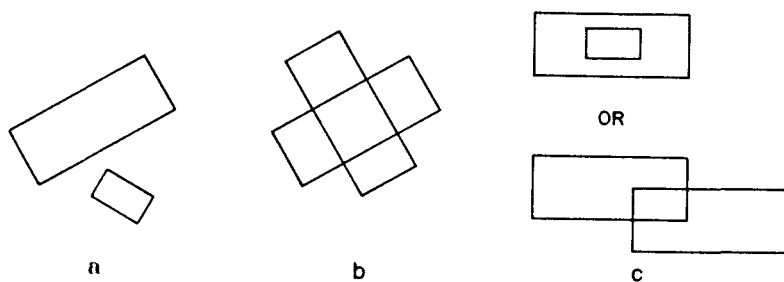
Figure 4.5 Three possible results of intersecting two strip trees: (a) null, (b) clear, (c) possible
