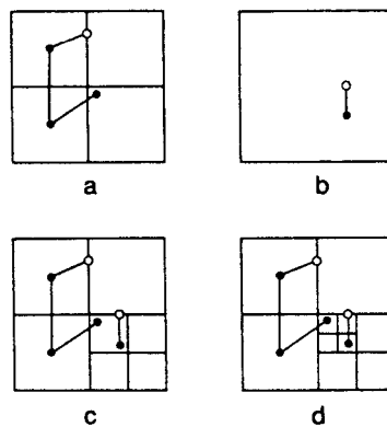
Figure 4.36 Insertion of a q -fragment into a PMR - f and PM_3 - f quadtree: (a) quadtree before insertion; (b) q -fragment being inserted; (c) the resulting PMR - f quadtree; (d) the resulting PM_3 - f quadtree. The cutpoints are shown with hollow circles, while the endpoints are shown with solid circles.
